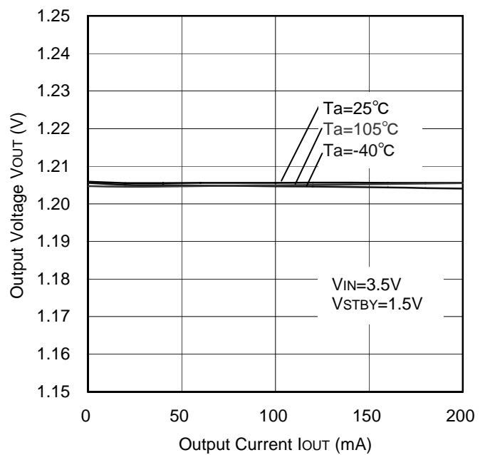
Figure 6. Load Regulation
