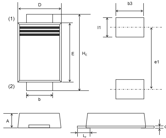
SOD-128, (PMD™)
