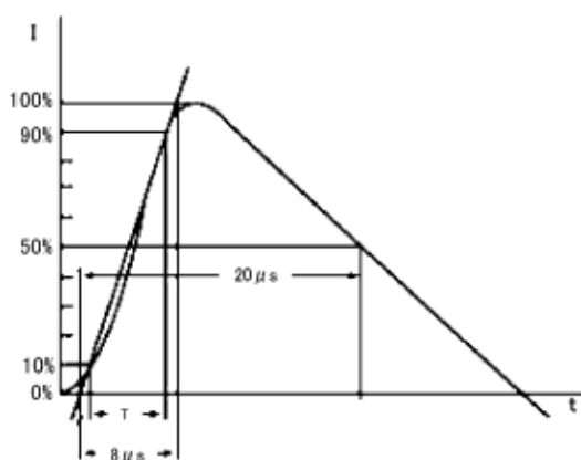
IEC61000-4-5 準拠 8/20 μs pulse
