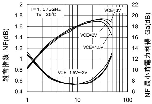
NF, Ga-Ic
