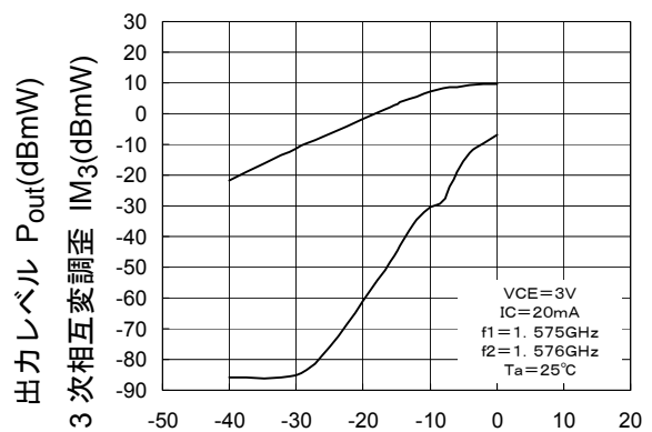
P_{out}, IM_3-P_{in}
