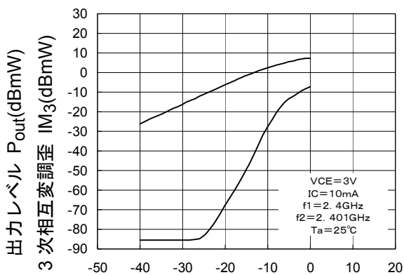
P_{out}, IM_3-P_{in}
