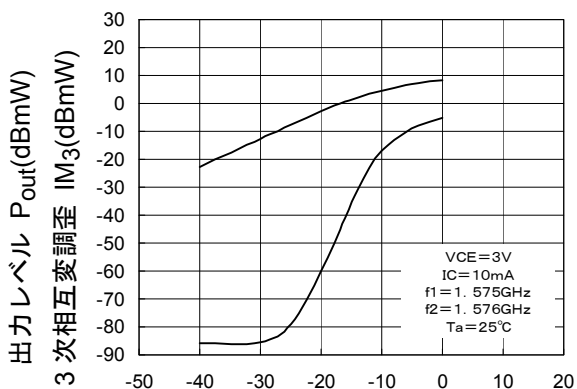
P_{out}, IM_3-P_{in}
