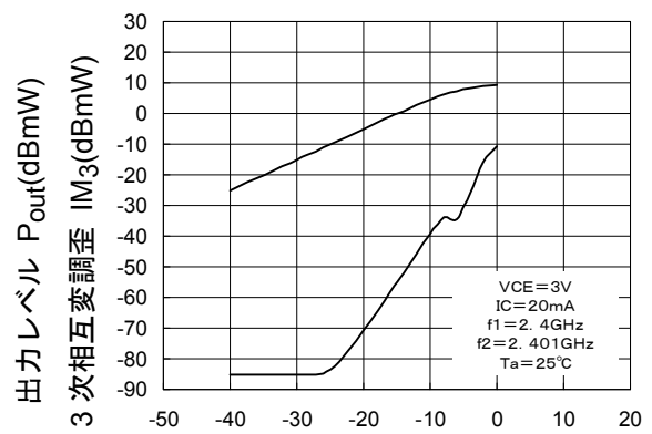
P_{out}, IM_3-P_{in}
