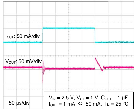
V OUT = 1.2V
