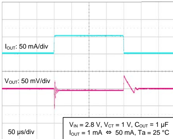
V OUT = 1.8V
