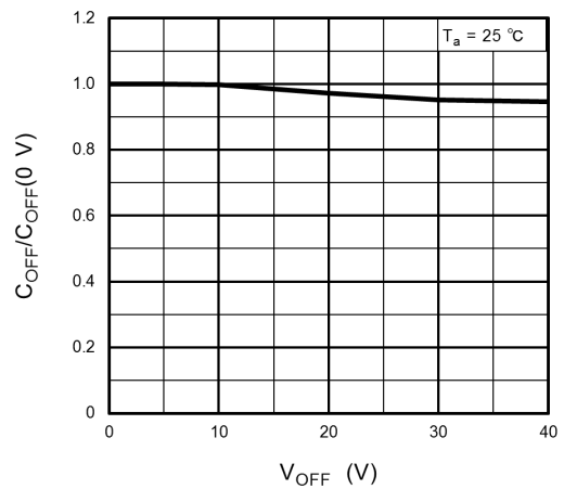
図 12.10 C_{OFF}/C_{OFF}(0\text{ V}) - V_{OFF}
