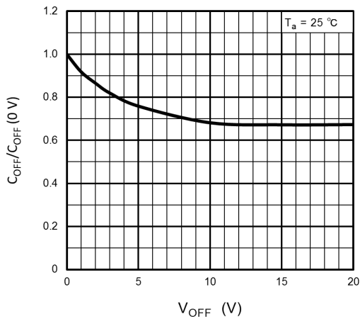
図 12.11 C_{OFF}/C_{OFF}(0V)-V_{OFF}
