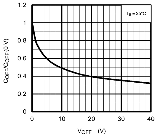
図 12.11 C_{OFF}/C_{OFF}(0V) - V_{OFF}
